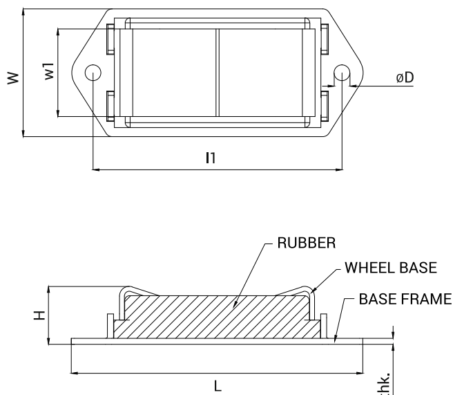
ANITVIBRATION PADS - TECHNICAL SPECIFICATIONS
